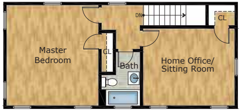
UPPER LEVEL
