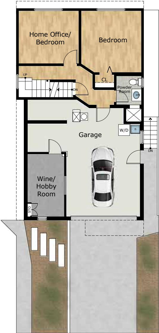
LOWER LEVEL
